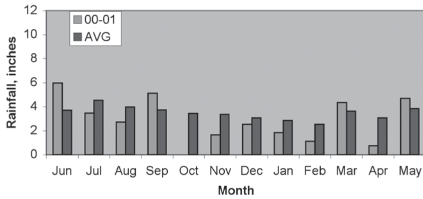
2000-01 Monthly Precipitation
