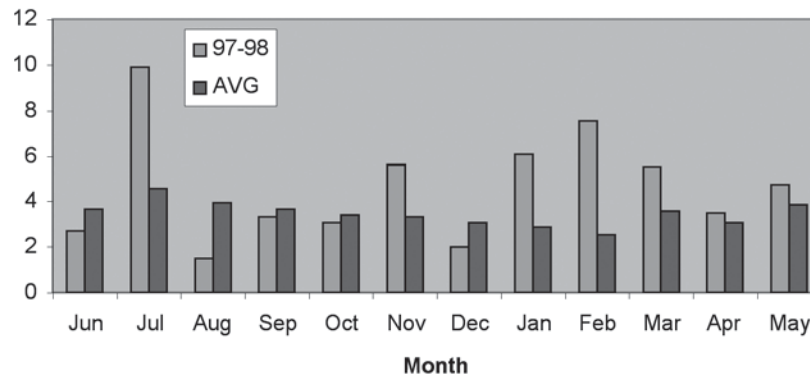
1997-98 Monthly Precipitation
