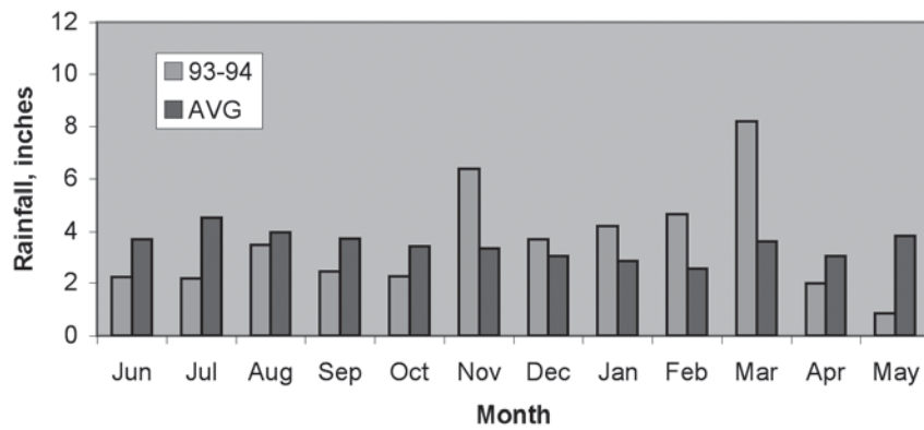
1993-94 Monthly Precipitation
