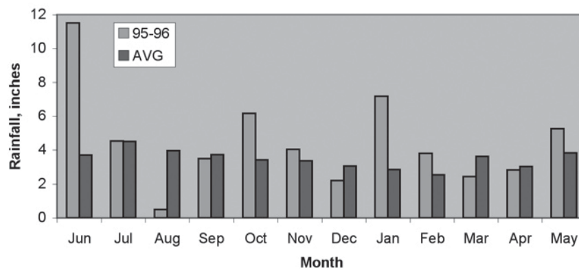
1995-96 Monthly Precipitation
