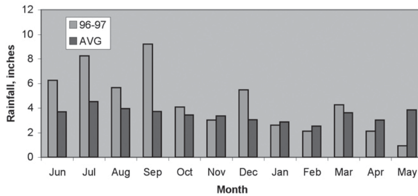
1996-97 Monthly Precipitation
