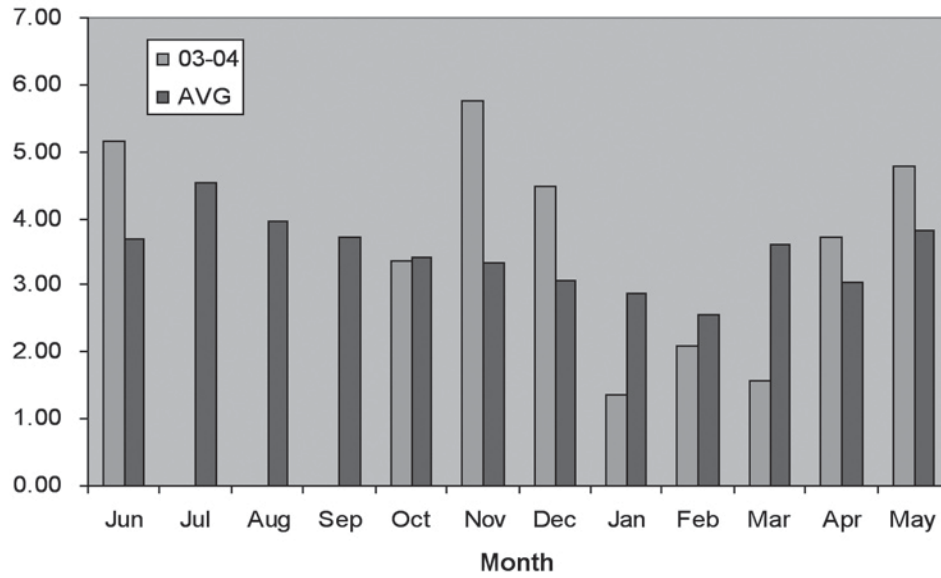
2002-03 Monthly Precipitation
