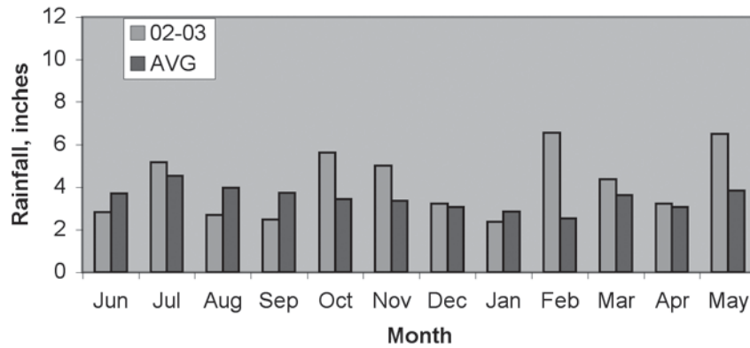
2002-03 Monthly Precipitation
