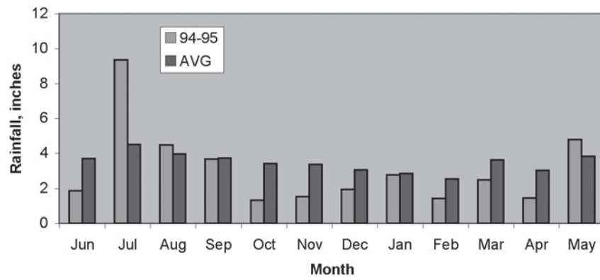
1994-95 Monthly Precipitation
