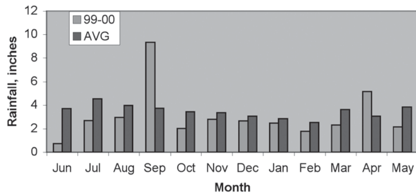
1999-00 Monthly Precipitation
