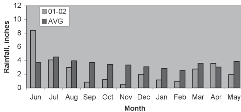
2001-02 Monthly Precipitation
