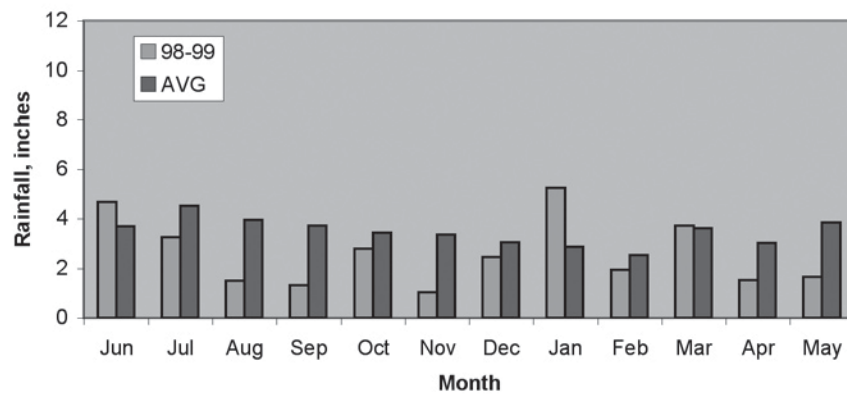
1998-99 Monthly Precipitation
